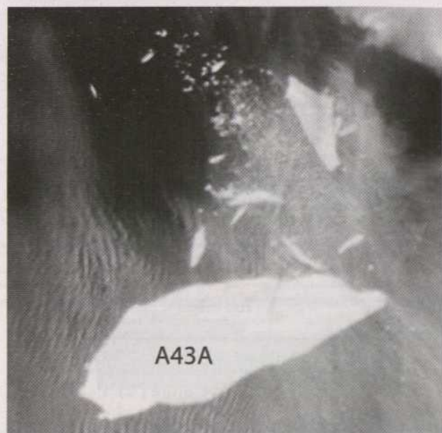
Fig. 7. MODIS image of A43A on 31 March 2005, showing rapid break-up after extensive summer surface melting. Image is 75 km on a side; location is near 50°S, 20°W. (Aqua MODIS image acquired 1530 UTC on 31 March 2005.)
