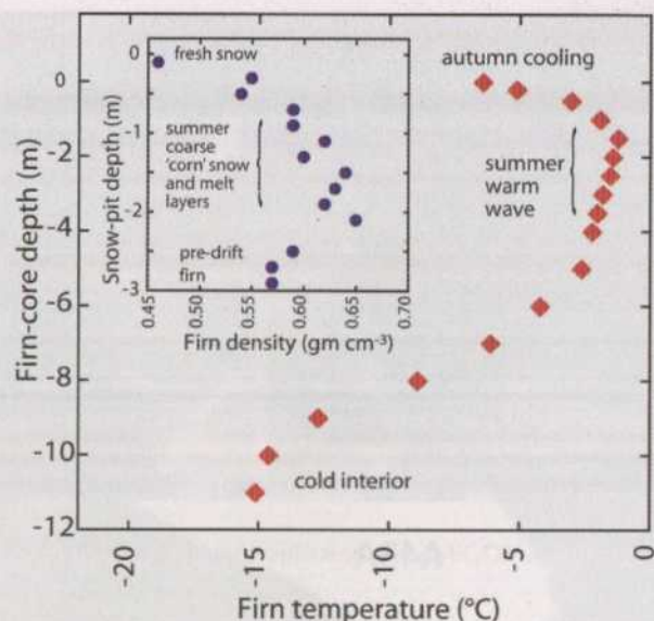
Fig. 6. Firn temperature from 11 m ice core taken at A22A during AMIGOS installation on 19 March 2006. Inset: firn-pit density on same date, adjacent to firn core. Temperature errors are \pm 0.5^{\circ}\text{C} ; firn density errors are \pm 0.03 \text{ g cm}^{-3} . 'Pre-drift' refers to the period prior to the rapid northward movement of A22A beginning in early 2005.
