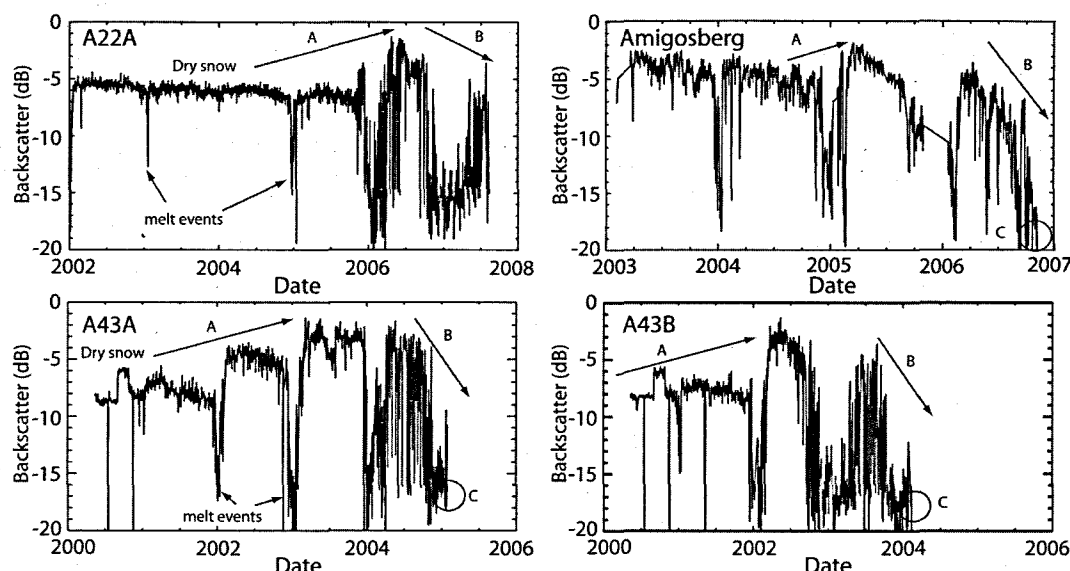
Fig. 12. Backscatter evolution of four of the icebergs in this study. Melt events are indicated by large abrupt drops in backscatter. Patterns of firn evolution with increasing melt are: (A) increasing backscatter after extended melt events in early evolution; (B) decreasing backscatter after refreeze as melt events become longer and more intense due to saturation of melt layers and specular reflection; and (C) rapid disintegration event as refrozen backscatter levels reach \sim 15 dB. A22A did not disintegrate during the period of observation. Amigosberg was not tracked for backscatter until March 2006. Backscatter 'events' of middle and late 2000 for A43A and A43B are sensor artifacts.
