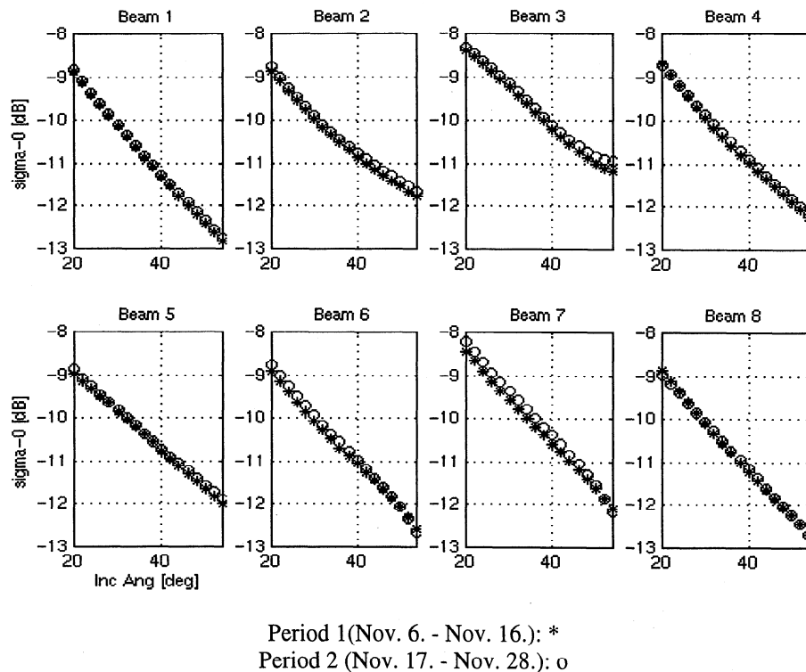
Figure 5. Time stability of NSCAT \sigma^0(\theta) response over Siberia for period 1, November 6–16 (stars), and period 2, November 17–28 (circles).
