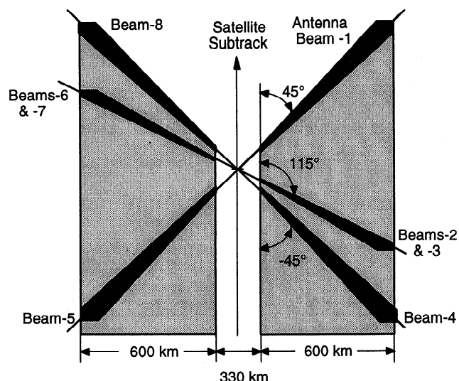
Figure 1. NASA scatterometer (NSCAT) antenna illumination patterns.
