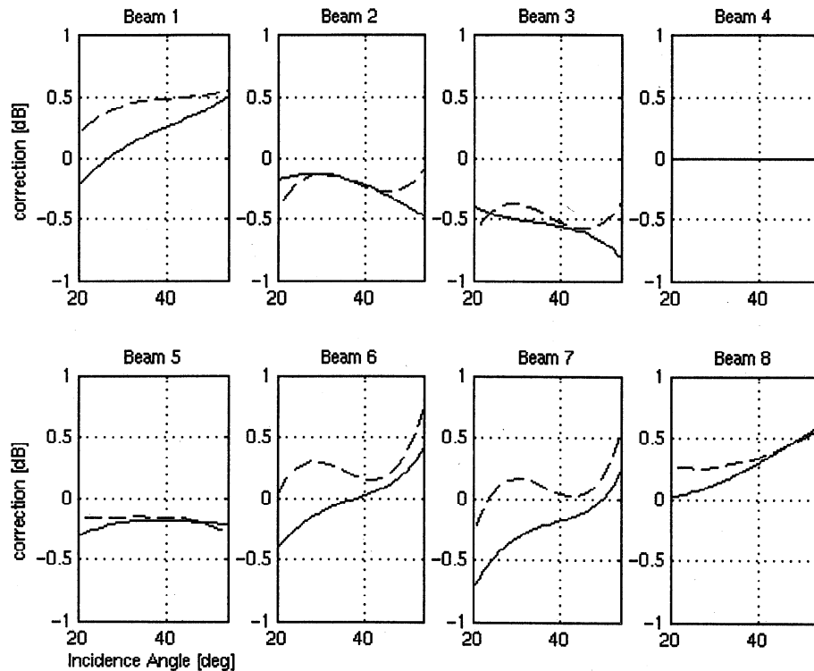
Figure 15. Comparison of NSCAT baseline, ocean-derived, and land-derived beam corrections for descending passes.
