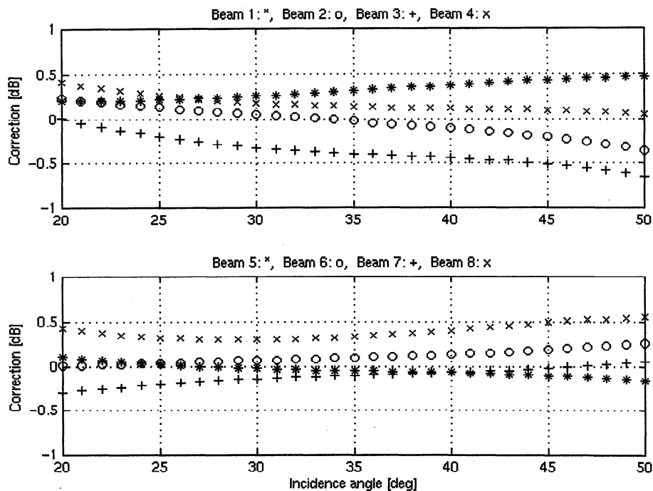
Figure 9. Beam corrections based on Amazon November 1996 data.
