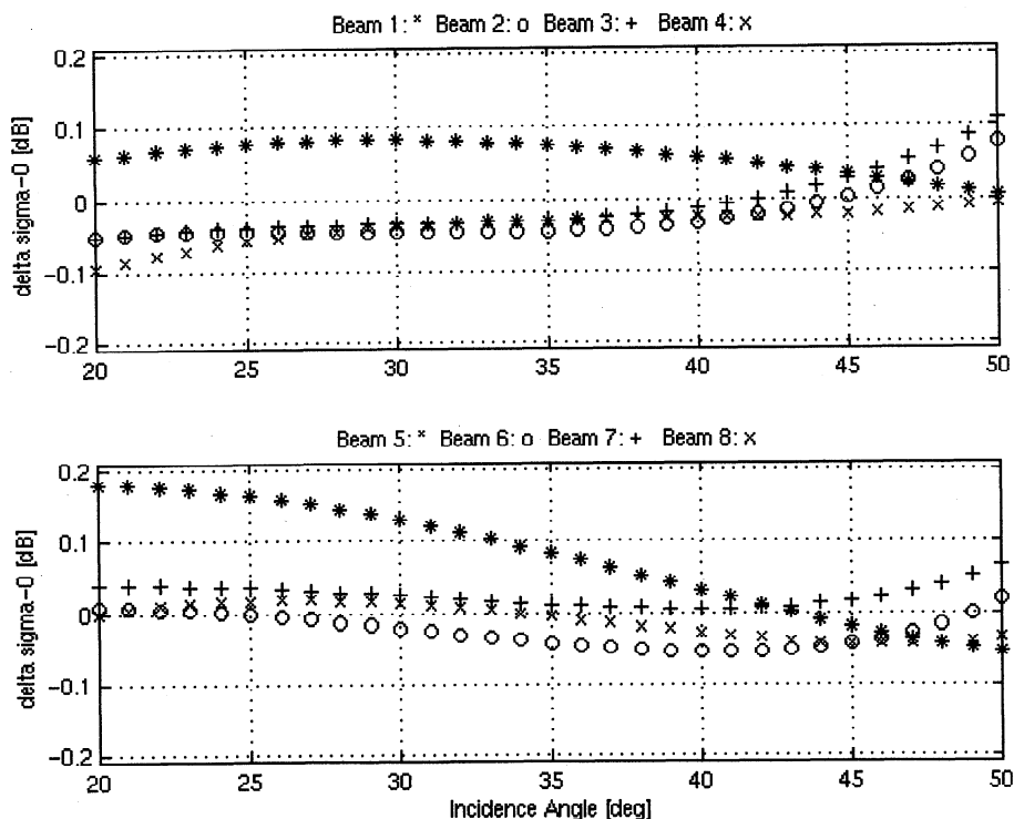
Figure 11. Differential beam corrections (November 96 - January 1997) from Amazon data.
