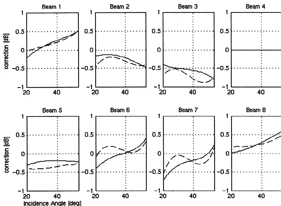
Figure 14. Comparison of NSCAT baseline, ocean-derived, and land-derived beam corrections for ascending passes.
