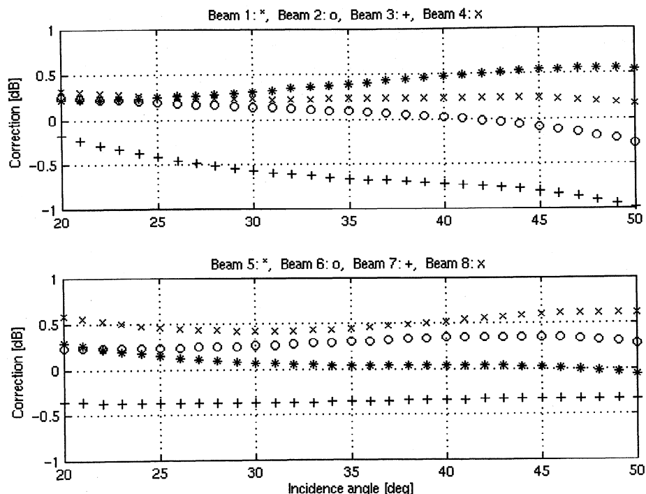
Figure 10. Beam corrections based on Siberia November 1996 data.
