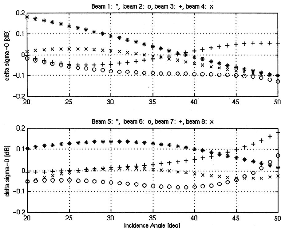
Figure 12. Differential beam corrections (November 96 - January 1997) from Siberian data.
