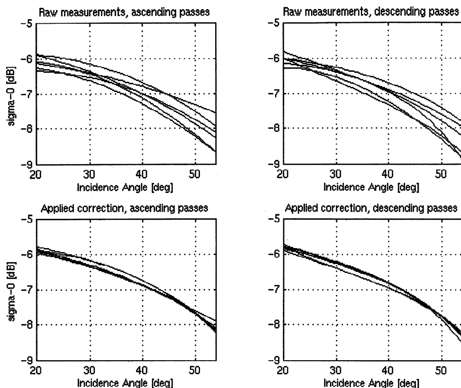
Figure 13. Effects of corrections on beam response for Amazon, November 1996.
