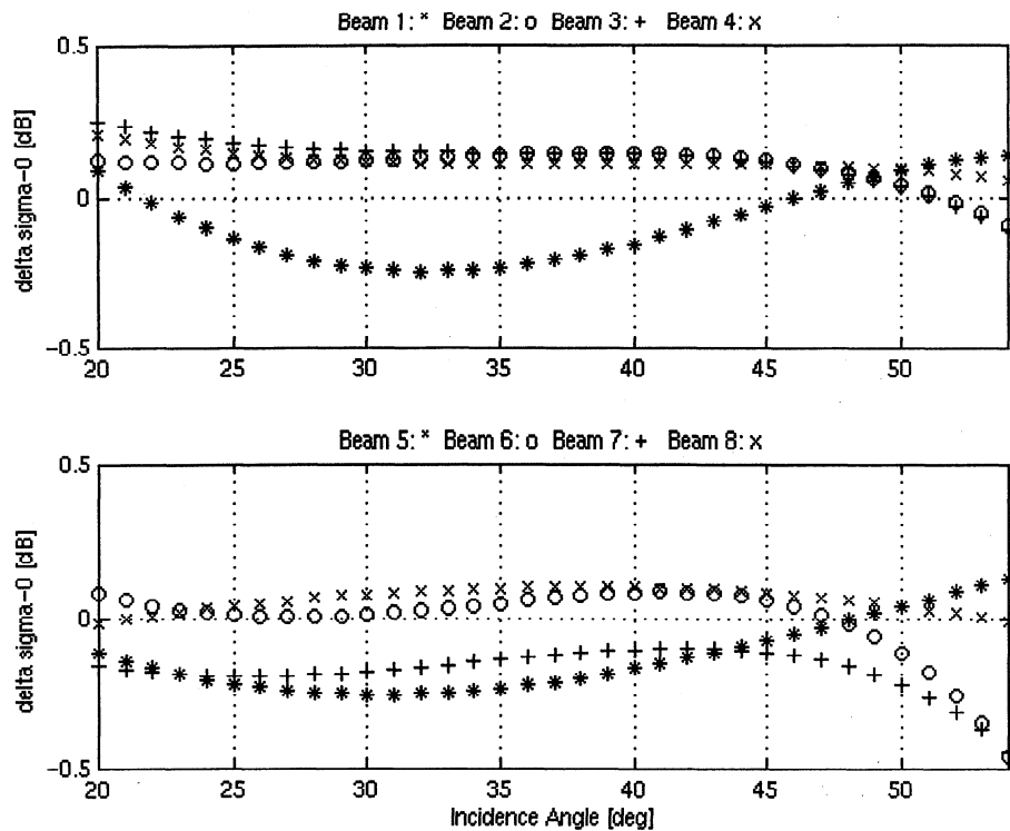
Figure 8. Differential beam corrections (ascending – descending revolutions) for Amazon, November 1996.
