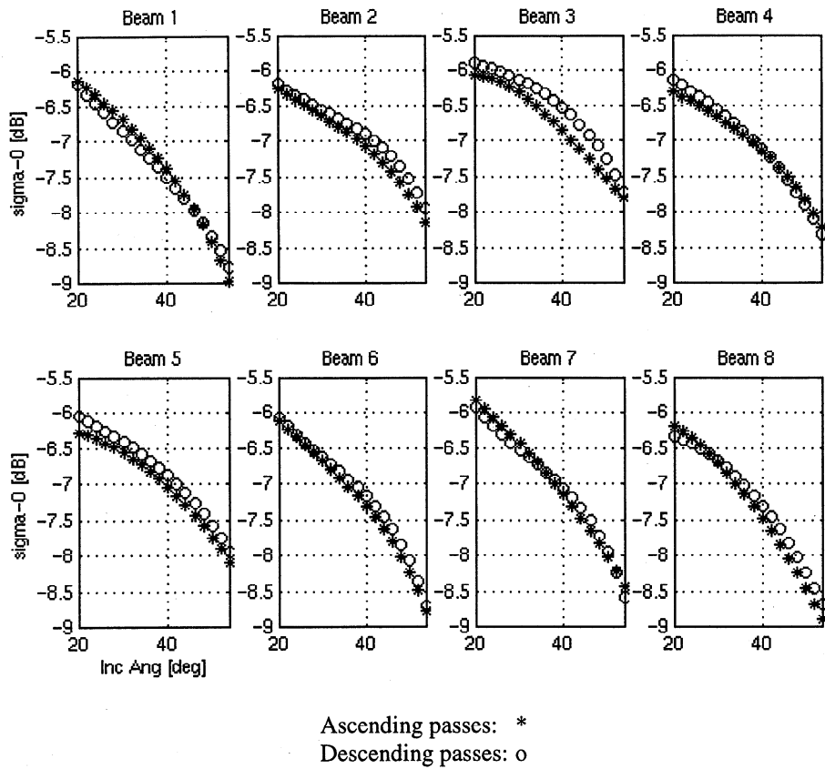
Figure 6. Diurnal effect of NSCAT \sigma^0(\theta) response over Amazon for ascending passes (stars) and descending passes (circles).
