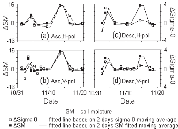
Fig. 2. Time series of the QuikSCAT enhanced Sigma-0 and station soil moisture temporal change detection analyses. The station data were used because of its higher temporal frequency as compared to the PLMR and AMSR-E products. This allowed achieving the maximum number of coincident observations with QuikSCAT overpasses.
