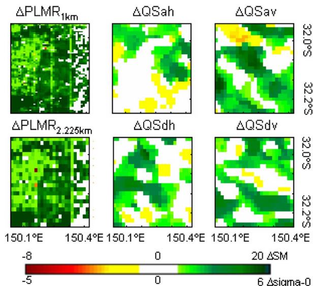
Fig. 3. Change analysis: Change in PLMR derived soil moisture and QuikSCAT sigma-0 from November 9 to 13 QS stands for QuikSCAT, a, d, h, and v indicate overpass (ascending or descending) and polarization (vertical or horizontal).
