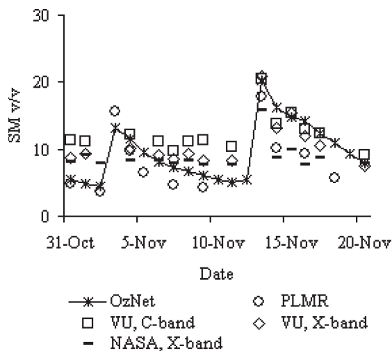
Fig. 1. Spatially averaged AMSR-E, PLMR, and OzNet station soil moisture time series for the duration of the NAFE'06 campaign over the 60 \text{ km} \times 40 \text{ km} Yanco sampling domain.
