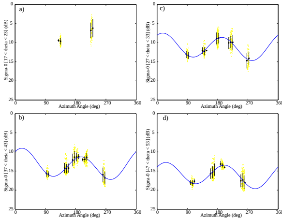
Fig. 6. Escat \sigma^o measurements at various incidence angles from area 5. Measurements are from \pm 3^\circ of the central incidence angle. Left to right, top to bottom, the central incidence angles are 20^\circ , 30^\circ , 40^\circ , and 50^\circ . The solid lines represent the second order azimuth fit (see text).
