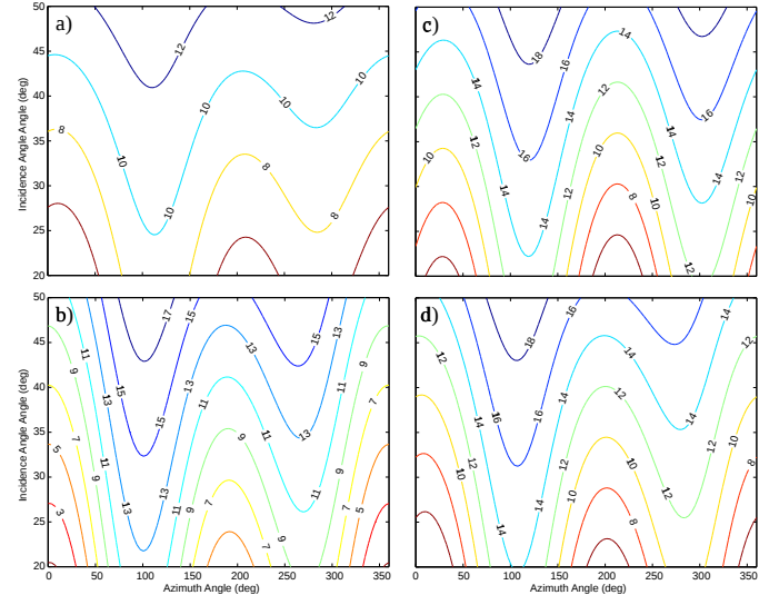
Fig. 9. Contour plots of \sigma^0(\theta, \phi_i) computed from the azimuth modulation model parameters estimated from V pol NSCAT data for study areas a) 5, b) 9, c) 8, and d) 11. For these areas \psi_0 is just to the right of the 100° azimuth angle.
