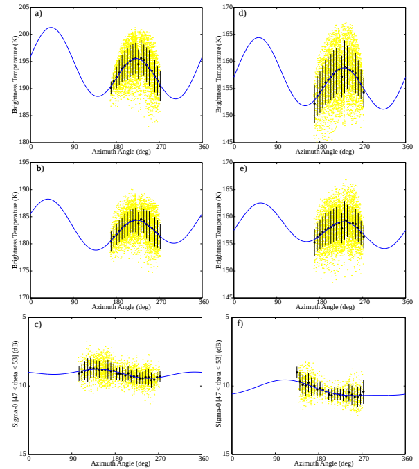
Fig. 5. Scatter plots of T_b and \sigma^0 versus azimuth angle for study area 2 - a) SSM/I 19v, d) SSM/I 19h, b) SSM/I 37v, e) SSM/I 37h, and NSCAT c) V pol, and f) H pol at 50^\circ incidence angle. In this and later figures, values are shown as gray dots, the means of \pm 3^\circ degree wide bins are shown as asterisks. The solid vertical lines indicate plus and minus one standard deviation about the mean. Scatterometer statistics are computed in dB. The solid lines represent the second order azimuth fit (see text).
