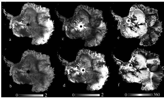
Fig. 10. NSCAT images from six days (JD 277-282,1996) NSCAT V pol \sigma^0 measurements: a) projection error standard deviation image prior to azimuth modulation removal, b) projection standard deviation image after azimuth modulation estimation, c) magnitude ( M_1 ) of the estimated first-order azimuth modulation harmonic term, d) magnitude ( M_2 ) of the estimated second-order azimuth modulation harmonic term, e) phase angle ( \phi_1 ) of the estimated first-order azimuth modulation harmonic term, f) phase angle ( \phi_2 ) of the estimated second-order azimuth modulation harmonic term. To produce this figure, the 4.45 km pixel resolution has been averaged down to 8.9 km resolution to reduce the image size and match the Escat image pixel resolution.
