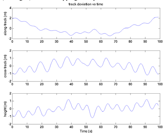
Fig. 2. Plots of the UAS displacement from ideal straight-line flight for a typical image during CASIE09 flights. The periodic variation is due to the UAS autopilot operation.
